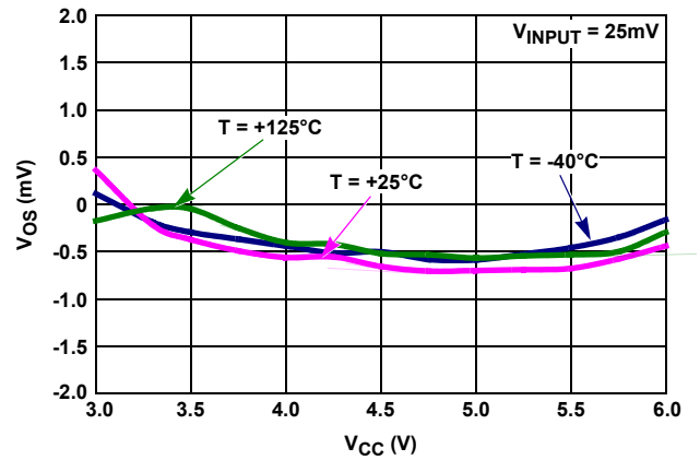
FIGURE 30. AUXILIARY V_{BUS} V_{OS} vs V_{CC}
