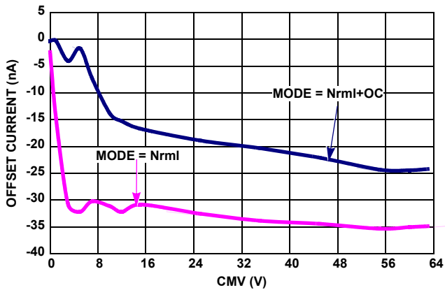
FIGURE 47. PRIMARY V_{SHUNT} OFFSET CURRENT vs COMMON MODE VOLTAGE
